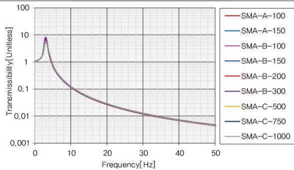
전달율 Graph
