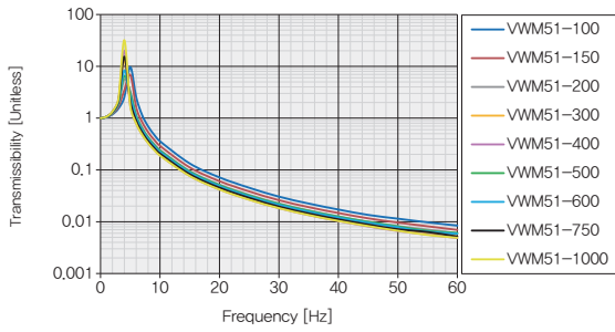
전달율 Graph
