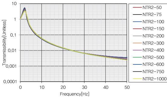
전달율 Graph
