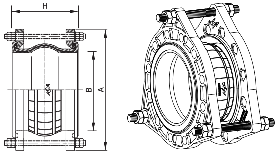
NFC10 (1 ball)
