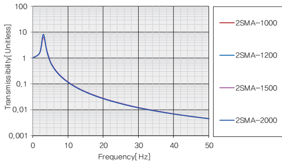
전달율 Graph
