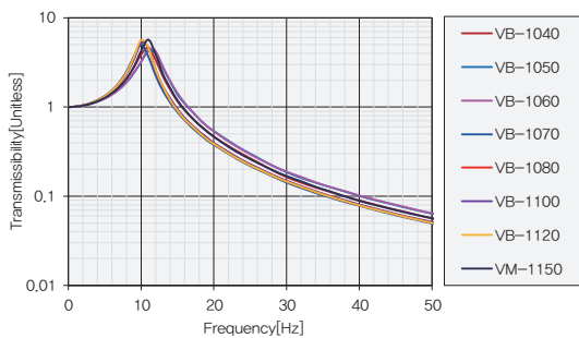
전달율 Graph
