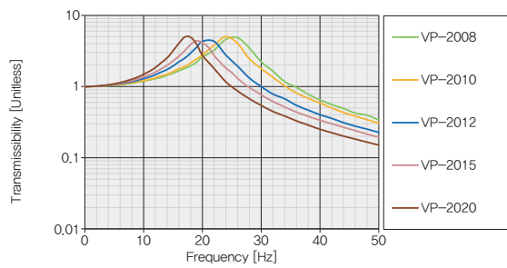
전달율 Graph
