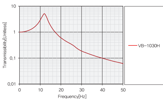
전달율 Graph
